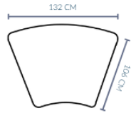
CURVED OTTOMAN
